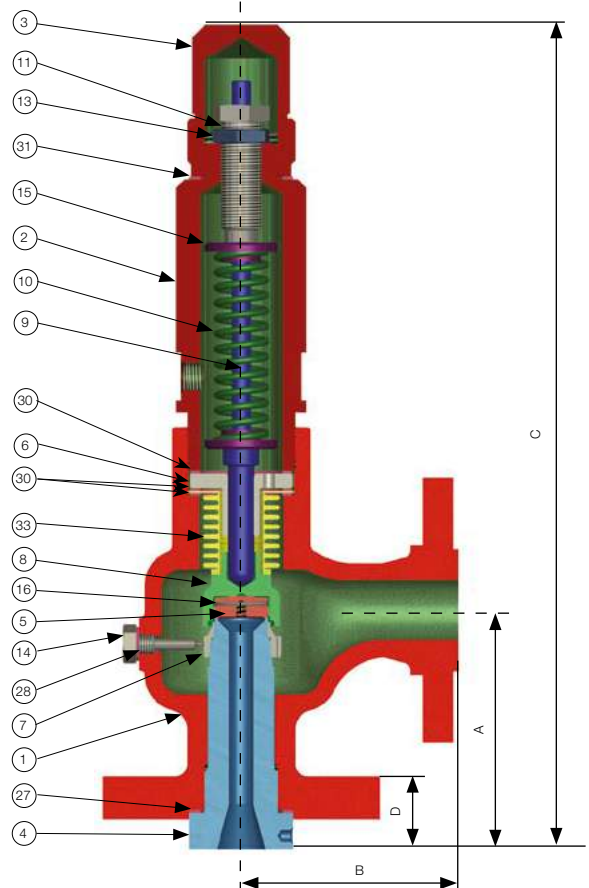
BELLOWS VALVE
