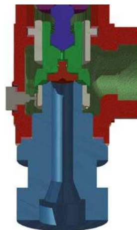
SOCKET WELDING
